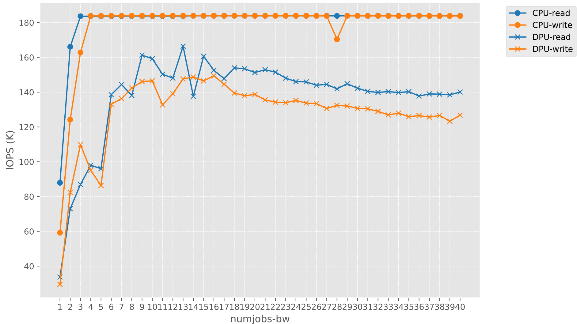
IOPS vs numjobs-bw (CPU vs DPU)
